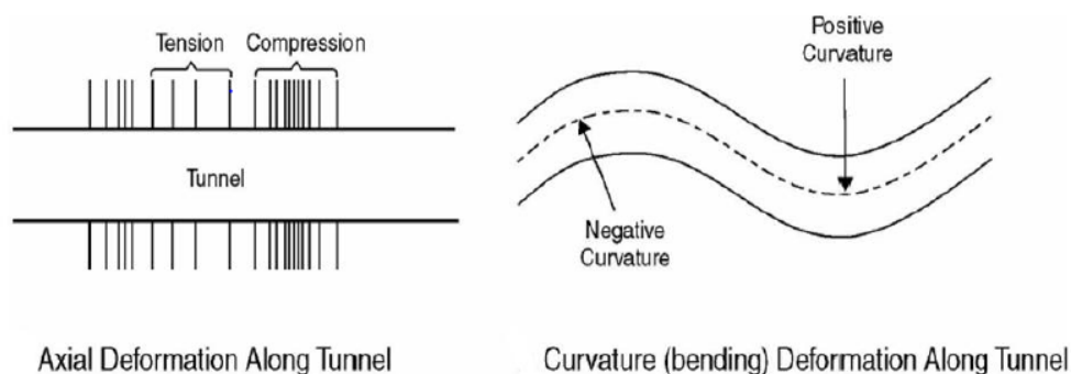
Figure 4.3: Axial and curvature deformations (from FHWA-NHI-11-032 (77) )
