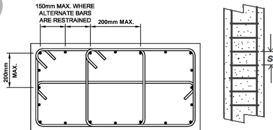
Figure 5.5: Rectangular column tie spacings
